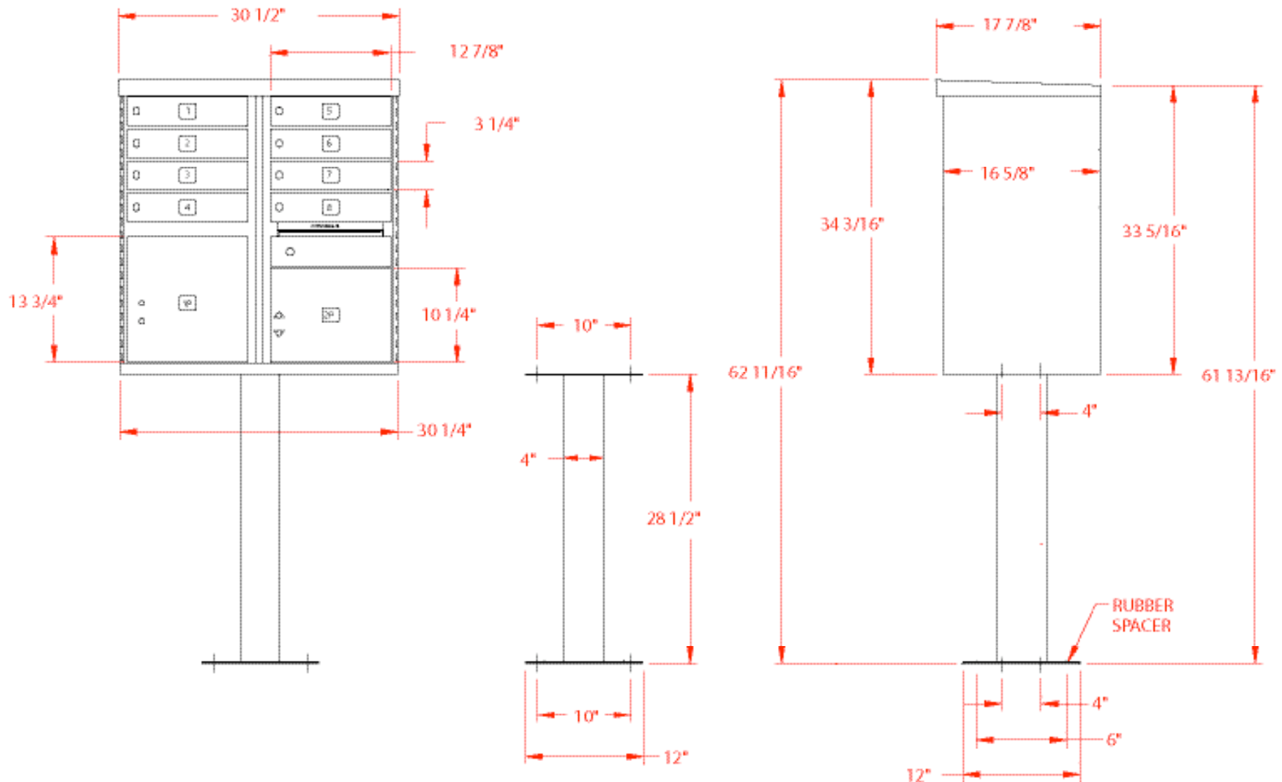
31" PEDESTAL
