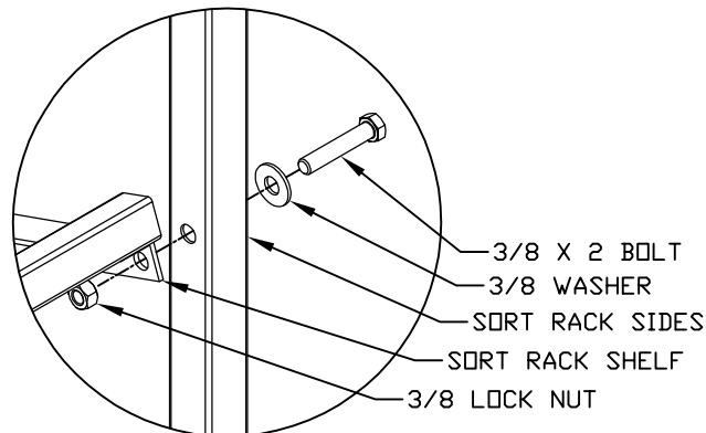
SHELF ASSEMBLY 4 PLACES PER SHELF
