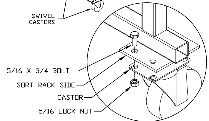
CASTOR ASSEMBLY 4 PLACES PER CASTOR (STANDARD AND SWIVEL)
